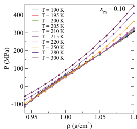
FIG. 5. EOS in the P - \rho isotherms plane of the x_m = 0.10 solution. The state points (diamonds) are shown for temperatures 190 \text{ K} \leq T \leq 220 \text{ K} every \Delta T = 5 \text{ K} , T = 250 \text{ K} , T = 280 \text{ K} , and T = 300 \text{ K} . The lines are obtained from the polynomial fits shown in Fig. 4.
