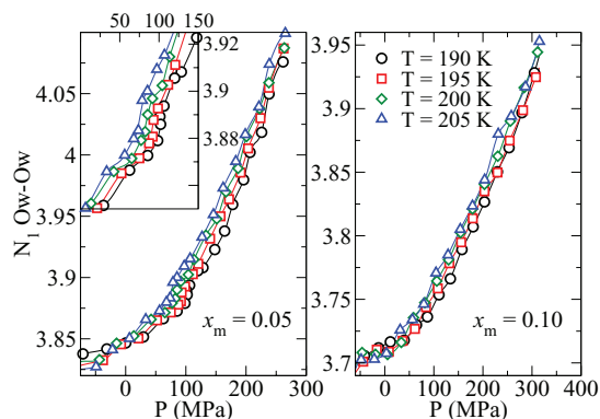
FIG. 8. Ow–Ow first shell coordination numbers N_1 calculated integrating the RDFs up to r = 3.2 \text{ \AA} as a function of pressure for the x_m = 0.05 (left) and x_m = 0.10 (right) solutions. The temperatures shown are T = 190 \text{ K} , T = 195 \text{ K} , T = 200 \text{ K} , and T = 205 \text{ K} . The inset of the left panel shows a magnification of the region close to the LLC of the x_m = 0.05 solution.
