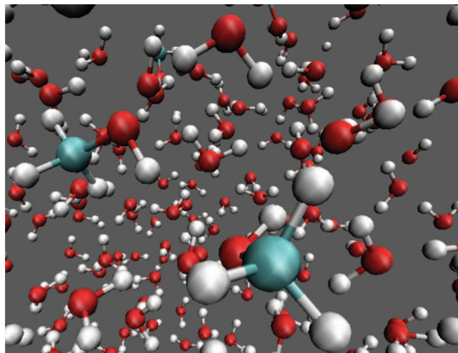
FIG. 1. Detail of two methanol molecules immersed in water taken from a blown-up snapshot of the x_m = 0.10 solution. For visualization purposes, only the atoms within a cube of 20 Å edge length in the center of the box are displayed. Atom color coding is: oxygen (red), hydrogen (white), and carbon (turquoise).
