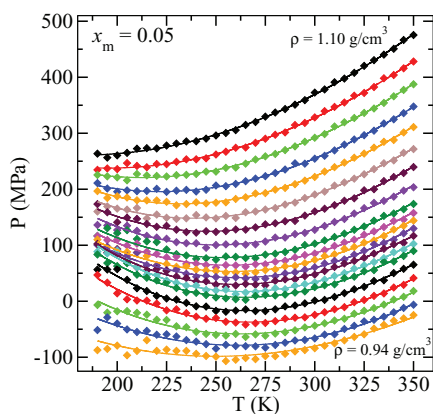
FIG. 2. EOS in the P - T isochores plane of the x_m = 0.05 solution. The state points reported (diamonds) span temperatures from T = 350 \text{ K} to T = 190 \text{ K} . The isochores shown are at densities, in \text{g/cm}^3 , 0.94 \leq \rho \leq 0.99 every \Delta\rho = 0.01 , \rho = 0.995 , \rho = 1.00 , \rho = 1.005 , \rho = 1.01 , \rho = 1.015 , and 1.02 \leq \rho \leq 1.10 every \Delta\rho = 0.01 (from bottom to top). The lines are fourth-degree polynomial fits to the simulated state points. The convergence of the isochores points to a LLCP located at 190 \text{ K} < T_c < 195 \text{ K} , 90 \text{ MPa} < P_c < 100 \text{ MPa} , and 1.00 \text{ g/cm}^3 < \rho_c < 1.005 \text{ g/cm}^3 .
