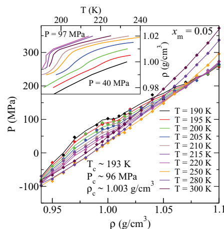
FIG. 3. EOS in the P - \rho isotherms plane of the x_m = 0.05 solution. The state points (diamonds) are shown for temperatures 190 \text{ K} \leq T \leq 220 \text{ K} every \Delta T = 5 \text{ K} , T = 250 \text{ K} , T = 280 \text{ K} , and T = 300 \text{ K} . The lines are obtained from the polynomial fits shown in Fig. 2. A horizontal inflection point develops between the T = 195 \text{ K} and the T = 190 \text{ K} isotherms. (Inset) Isobars obtained performing horizontal cuts on the polynomial fits shown in Fig. 2 for pressures, in MPa, P = 40, 50, 60, 70, 80, 85, 91.5, 95, 97 (from bottom to top). A vertical inflection point is observed between the P = 95 \text{ MPa} and P = 97 \text{ MPa} isobars. The behavior of the isotherms and the isobars is consistent with a LLCP at T_c \simeq 193 \text{ K} , P_c \simeq 96 \text{ MPa} , and \rho_c \simeq 1.003 \text{ g/cm}^3 .
