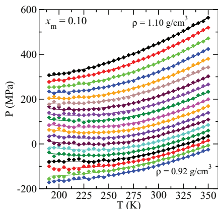
FIG. 4. EOS in the P - T isochores plane of the x_m = 0.10 solution. The state points reported (diamonds) span temperatures from T = 350 K to T = 190 K. The isochores shown are at densities, in g/cm 3 , 0.92 \leq \rho \leq 1.10 every \Delta\rho = 0.01 (from bottom to top). The lines are fourth-degree polynomial fits to the simulated state points. No point of convergence of the isochores is observed in the spanned region.
