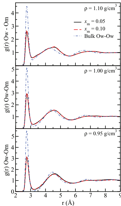
FIG. 9. Water oxygen–methanol oxygen (Ow–Om) RDFs at T = 190 \text{ K} and at \rho = 1.10 \text{ g/cm}^3 (top), \rho = 1.00 \text{ g/cm}^3 (middle), and \rho = 0.95 \text{ g/cm}^3 (bottom) for the x_m = 0.05 (solid line) and x_m = 0.10 (dashed line) solutions. For comparison the bulk water oxygen–oxygen (Ow–Ow) RDFs (dotted-dashed lines) at the corresponding densities are also shown.
