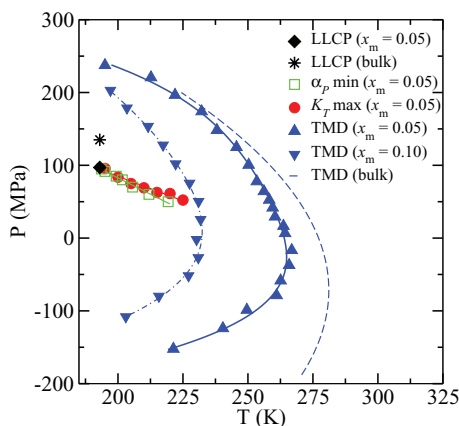
FIG. 6. Shown is the position of the LLCP in the x_m = 0.05 solution (diamond), estimated using Figs. 2 and 3, compared to the LLCP in TIP4P/2005 bulk water (star). 25 The line of extrema of the coefficient of thermal expansion \alpha_P (squares) and of the isothermal compressibility K_T (circles) converge at the LLCP. The TMD points calculated for x_m = 0.05 (triangles up) and x_m = 0.10 (triangles down) are also compared with the TMD line of TIP4P/2005 bulk water obtained by fitting the points calculated in Refs. 25 and 56 (dashed line).
