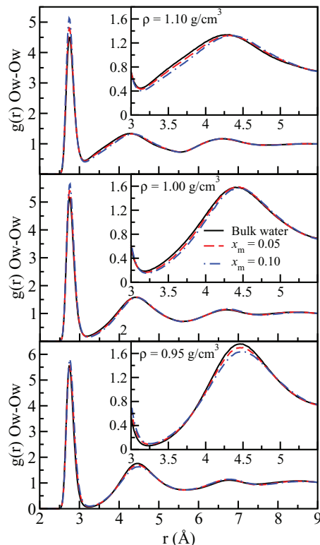
FIG. 7. Water oxygen-water oxygen (Ow–Ow) RDFs at T = 190 K and at \rho = 1.10 g/cm 3 (top), \rho = 1.00 g/cm 3 (middle), and \rho = 0.95 g/cm 3 (bottom) for bulk water (solid line), and the x_m = 0.05 (dashed line) and x_m = 0.10 (dotted-dashed line) solutions. The insets show a magnification of the region close to the second shell.
