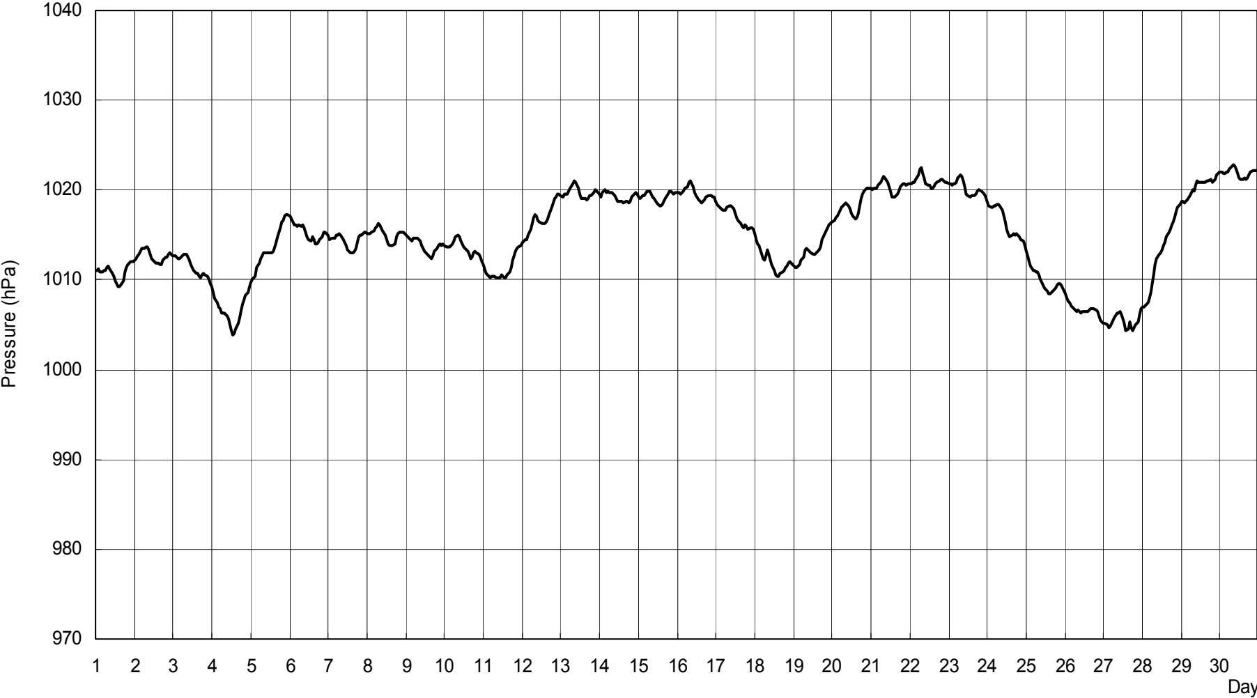
S.V.I.R.CO. Observatory - Pressure in hectoPascal - September 2007
