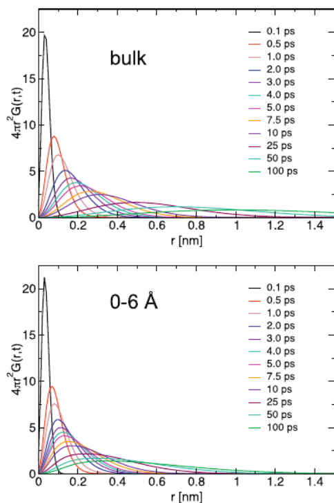
Fig. 6. Short time behavior of SVHFs. Upper panel: bulk water. Lower panel: hydration water. The temperature is 300 K. (For interpretation of the references to color in this figure legend, the reader is referred to the web version of this article.)
