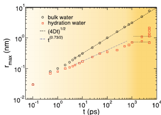
Fig. 8. Time behavior of the position of the maxima of SVHFs for hydration water and bulk water at 300 K. The darker yellow region is dominated by hopping processes
