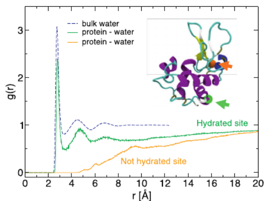
Fig. 2. RDF of water oxygen and a selected atom of the lysozyme, showing the difference between choosing an exposed/hydrated site/atom (green curve) and an inner/non-hydrated site/atom (orange curve). For comparison also the oxygen-oxygen RDF of bulk water is reported. The temperature is 300 K. In the inset, we show the location of the two selected sites of the lysozyme protein highlighted as balls superimposed to its secondary structure. The color of the arrow coincides with the color of the corresponding RDF. (For interpretation of the references to color in this figure legend, the reader is referred to the web version of this article.)
