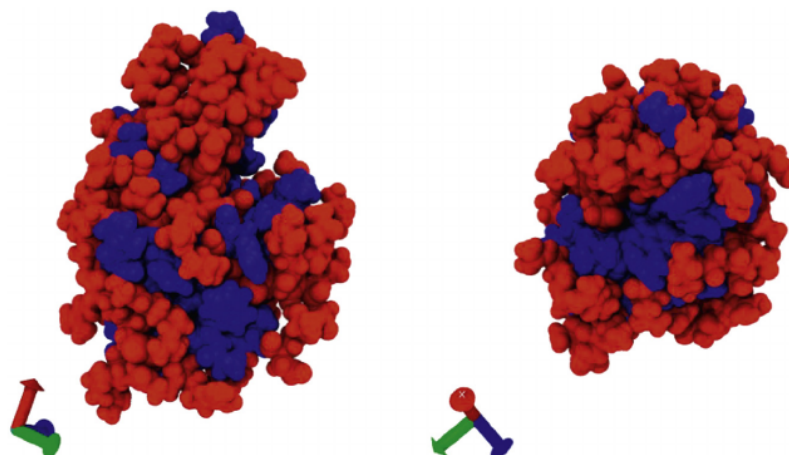
Fig. 1. Lysozyme in the Van der Waals representation, colored according to the hydrophobicity of its residues. Blue indicates hydrophobic residues, red indicates hydrophilic residues. (For interpretation of the references to color in this figure legend, the reader is referred to the web version of this article.)
